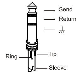
1/4" TRS insert
