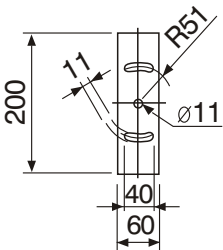
[Dimensions of bracket mounting holes]
